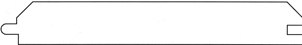
MCC110TG 3/4" x 5-1/4"
