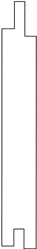
MCC109SI 3/4" x 5"
