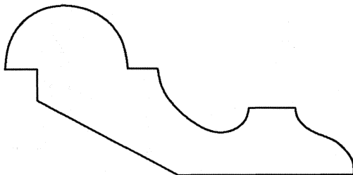
MCC103RPB 1-1/4" x 2-5/8"
