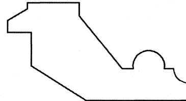
MCC130RPB 1" x 1-7/8"
