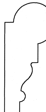
MCC105PIM 7/8" x 2"
