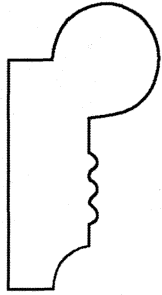
MCC100PIM 3/4" x 1-1/2"
