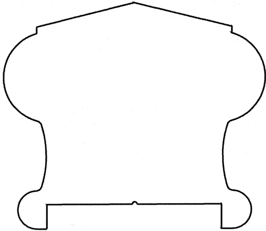
MCC119HR 2-1/4" x 2-5/8"
