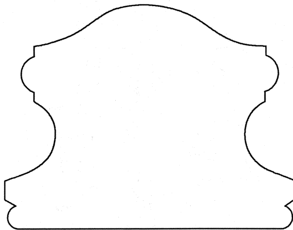
MCC112HR 2-5/16" x 2-15/16"
