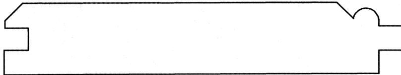
MCC102FPF From 5/8" to 3/4" x Any Face up to 8-1/2"
