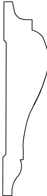
MCC121CHR 7/8" x 3-7/8"
