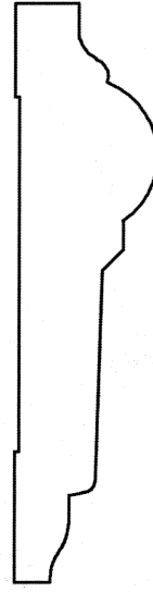
MCC120CHR 11/16" x 2-3/4"
