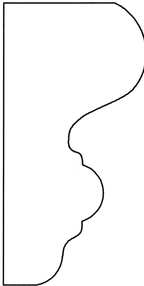
MCC116CHR 1-1/2" x 3"
